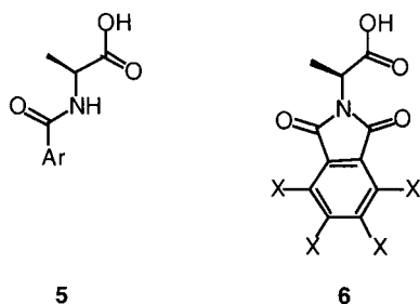
Figure. Resolving agents tested for the separation of 2,3-dibromopropan-1-ol (Ar = 3,4,5-triiodophenyl, 3,5-dinitrophenyl, [1,1'-biphenyl]-4-yl; X = Cl, Br)
